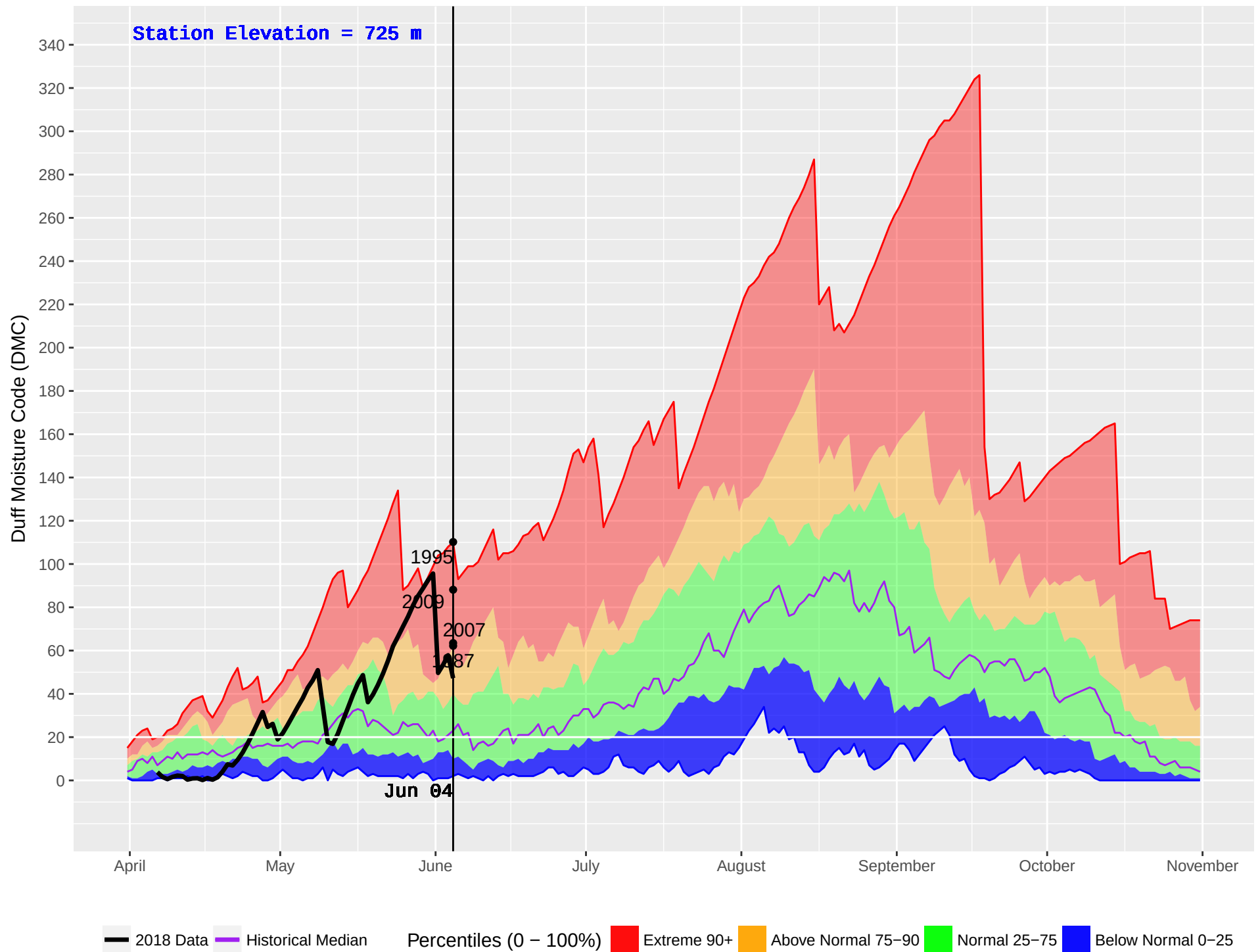
PENDOREILLE (402) : Historical (1986–2016) and Current (2018) Noon Duff Moisture Code (DMC)
