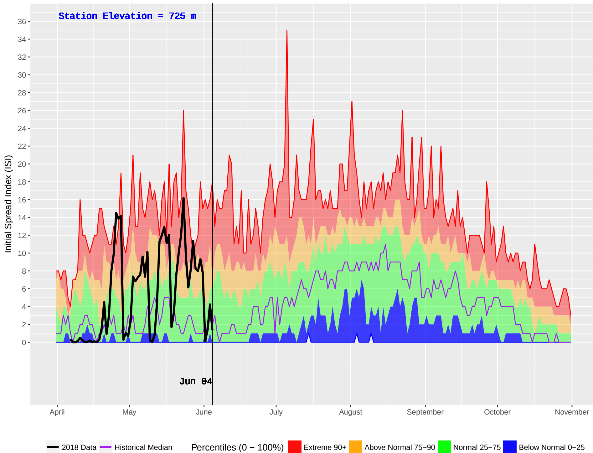
PENDOREILLE (402) : Historical (1986–2016) and Current (2018) Noon Initial Spread Index (ISI)
