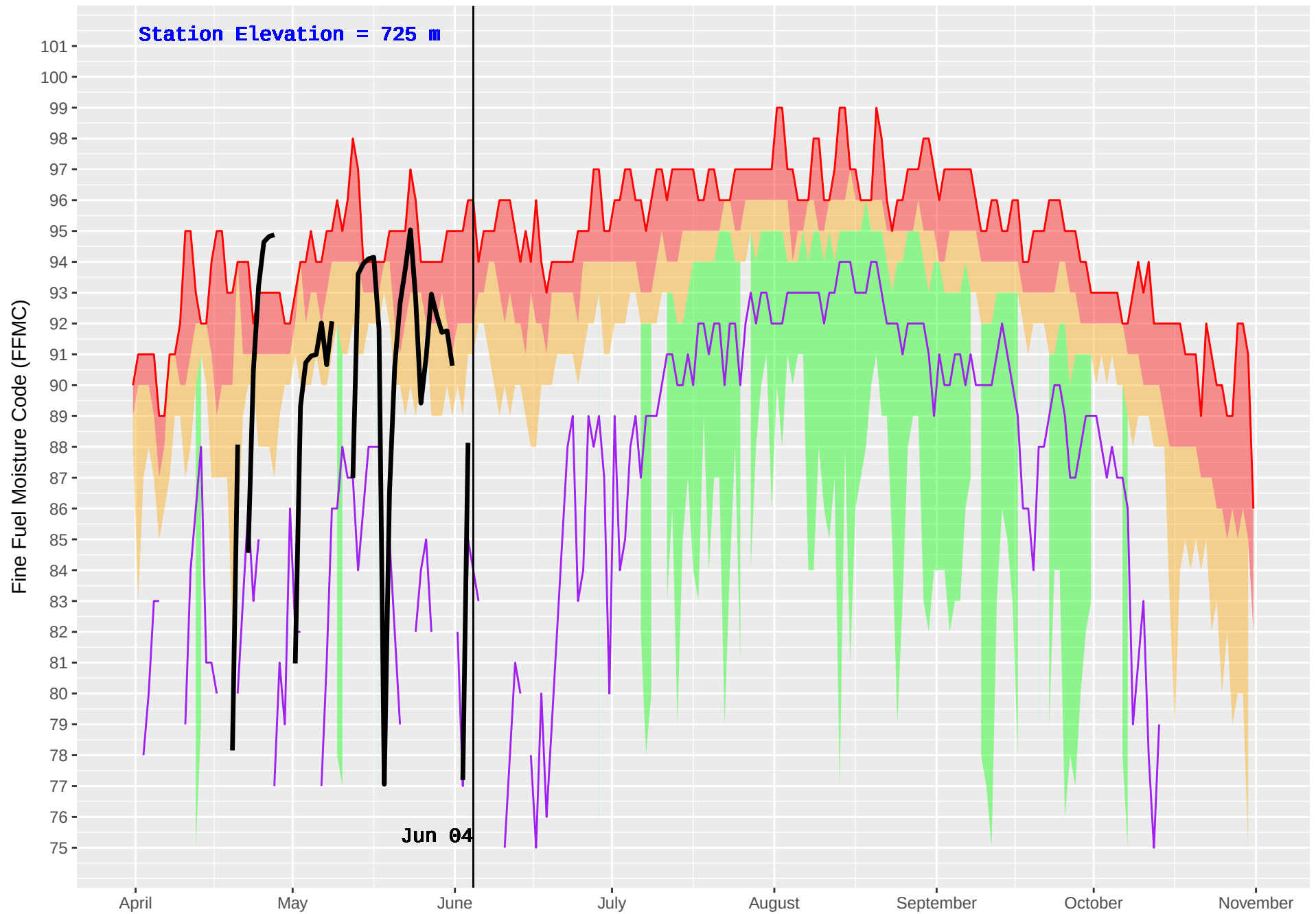
PENDOREILLE (402) : Historical (1986–2016) and Current (2018) Noon Fine Fuel Moisture Code (FFMC)
